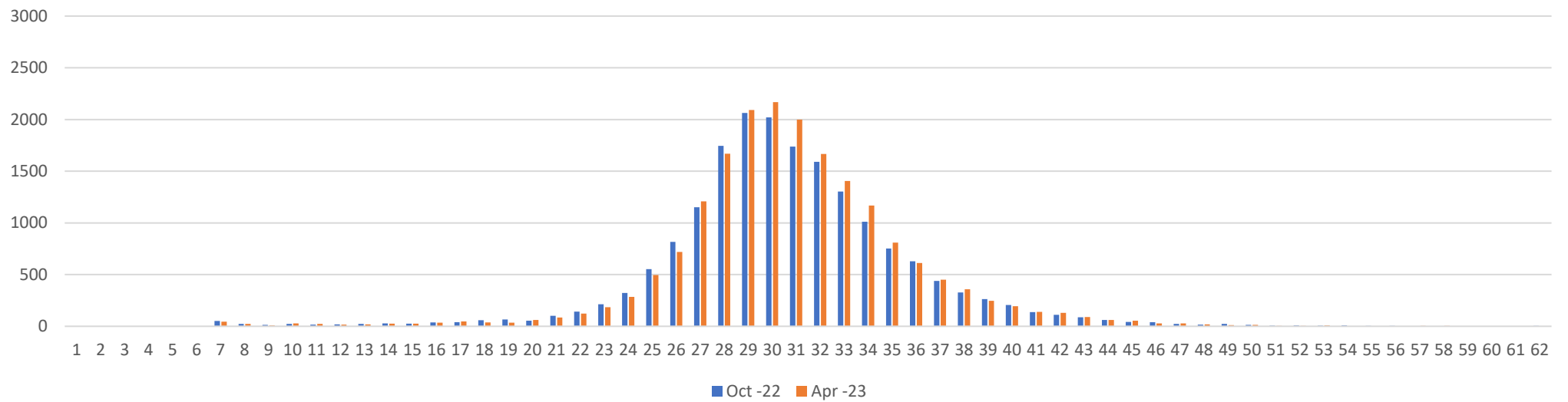
Total volume of traffic recorded against speed in mph in period travelling towards Beckley
