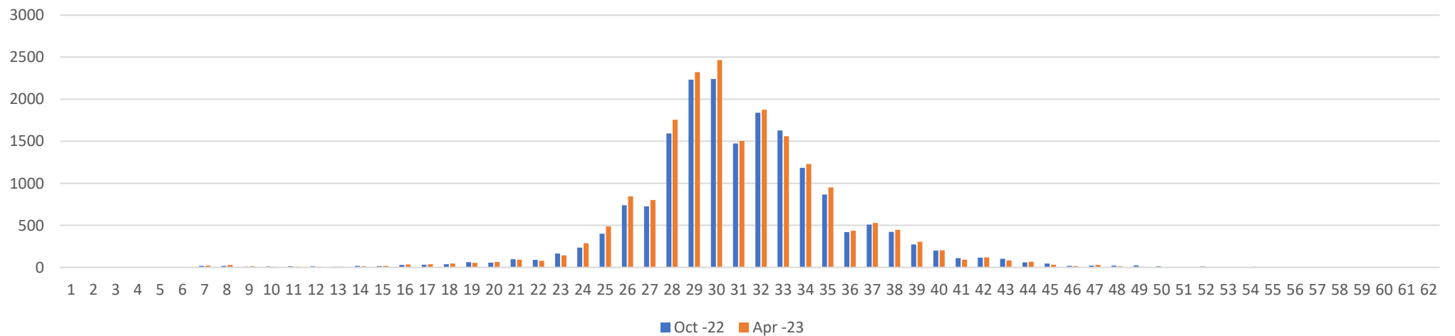
Total volume of traffic recorded against speed in mph in period travelling towards Rye
